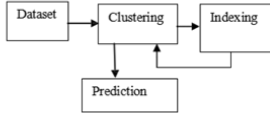
Fig. 1 System Architecture
