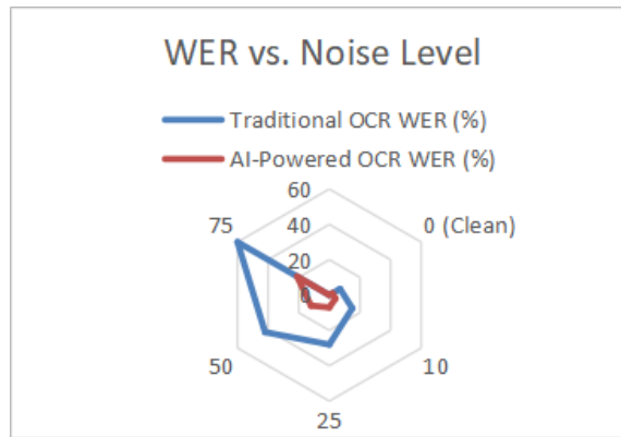
Fig. 4 WER vs. Noise Level
