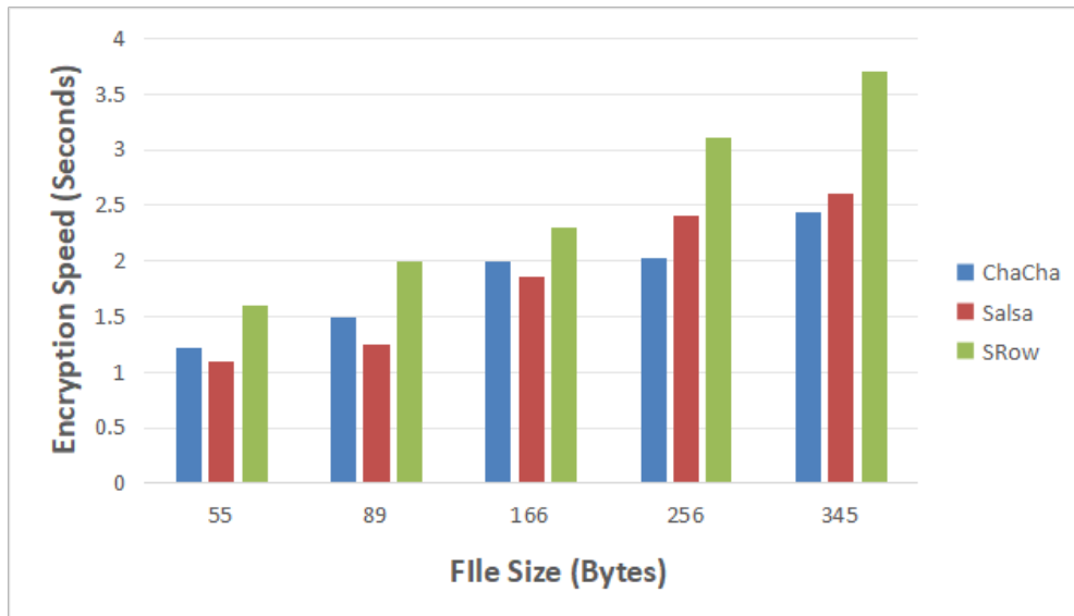
Fig. 5 ChaCha Vs Salsa Vs SRow Encryption Speed
