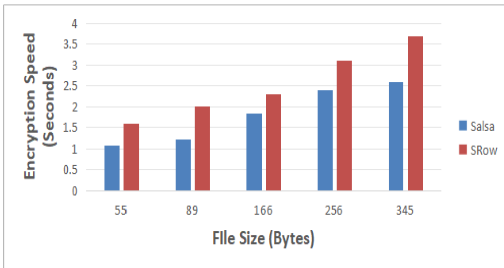
Fig. 4 Salsa Vs SRow Encryption Speed
