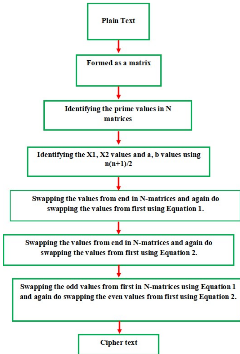
Fig. 1 KRB22 Methodology
