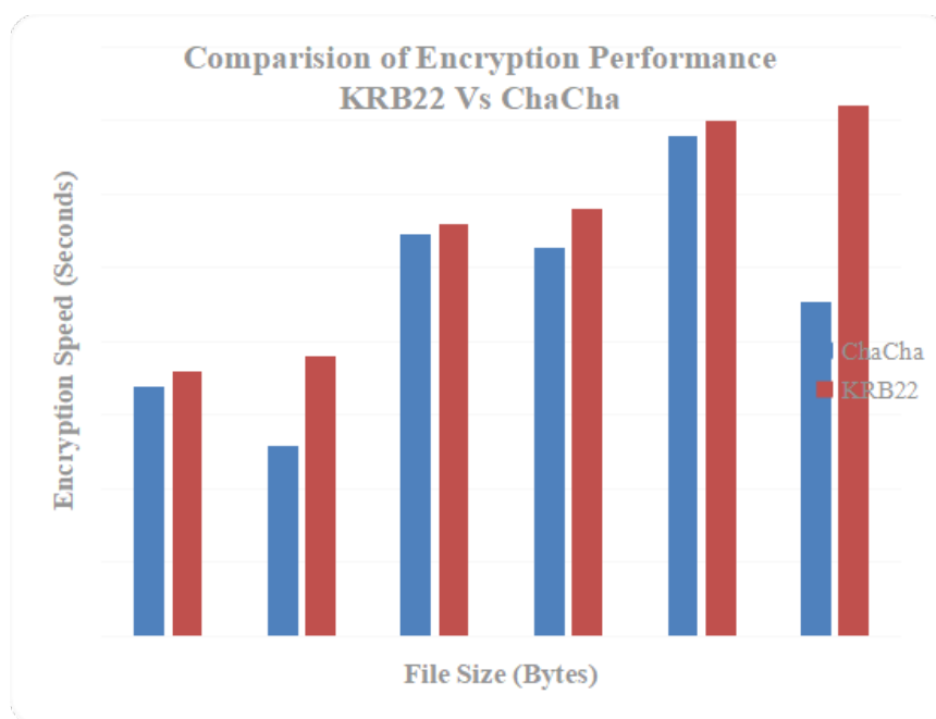
Fig. 2 Encryption performance
